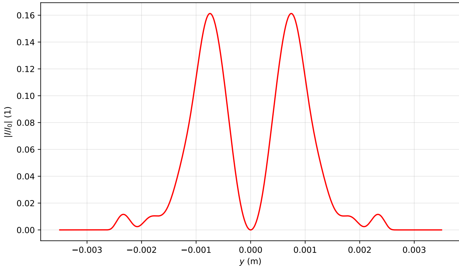
Intensity profile I(x=0, y, z=3.105)/I_0 , \text{Pin}=4.0\text{Pcr} , artificial time
